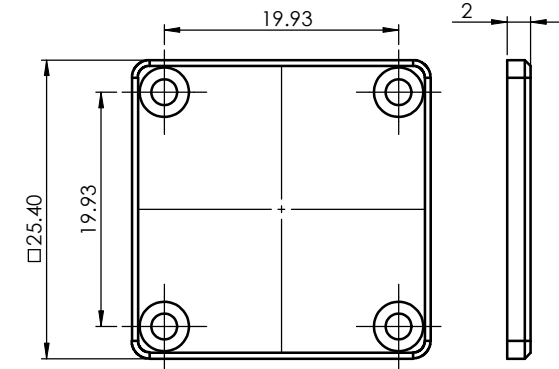
ASSEMBLY BOARD
