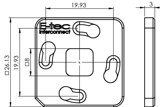
RETENTION FRAME
