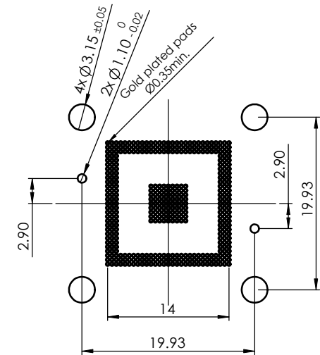
PCB LAYOUT
