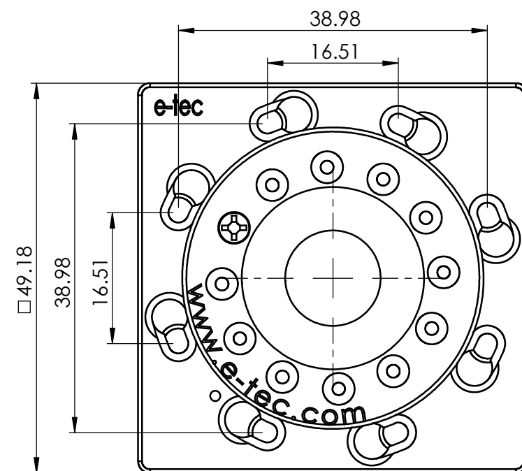
RETENTION FRAME
