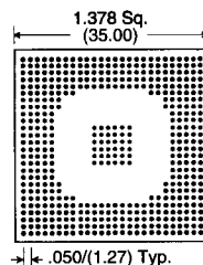
Footprint 476
